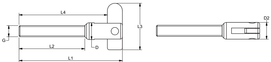
The dropnose is used with the small stainless steel bodies. Also available as terminal for 4 mm and 5 mm wire.
