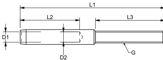
Blue Wave's small thread terminals.
