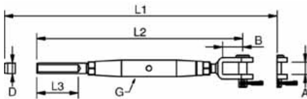
A short version of our classic rigging screw with small terminal.
